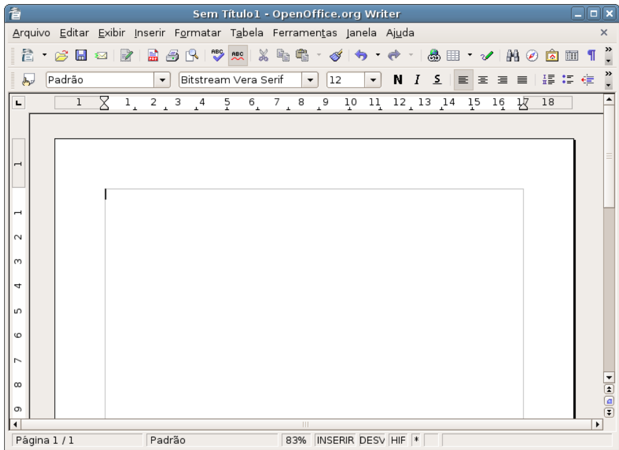
Ilustração 61: OpenOffice Writer
